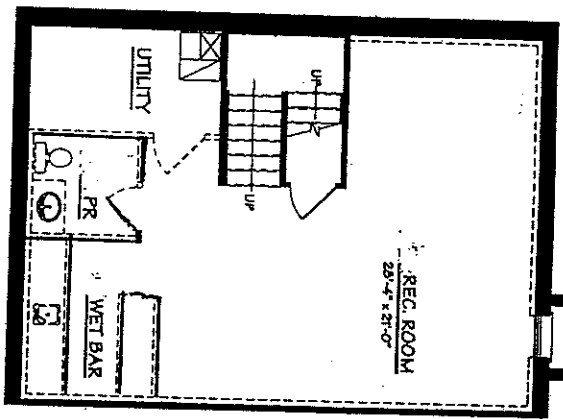
Basement Plan
