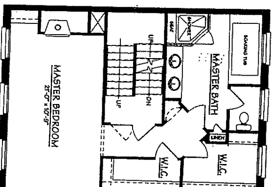
Floor Level 2 Plan
