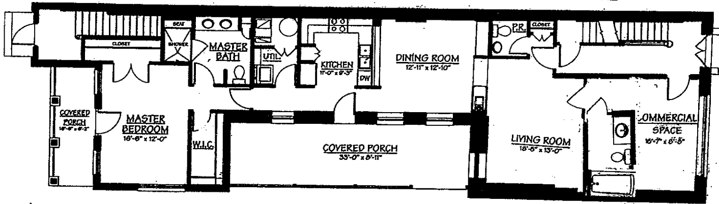
Floor Level 1-135-A
